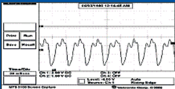
Six good injectors on a Jeep Cherokee capture
